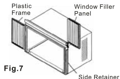
Side Retainer
